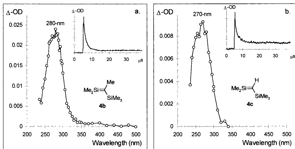
Figure 3. Transient UV absorption spectra, from far-UV (193 nm) laser flash photolysis of bis(trimethylsilyl)ketene ( 6b ; a) and pentamethyldisilylketene ( 6c ; b) in deoxygenated hexane and isooctane solution, respectively, at 23 °C. The spectra were recorded 0.1–1.0 μs after laser excitation. Typical decay traces, recorded at a monitoring wavelength of 255 nm, are shown as inserts.
